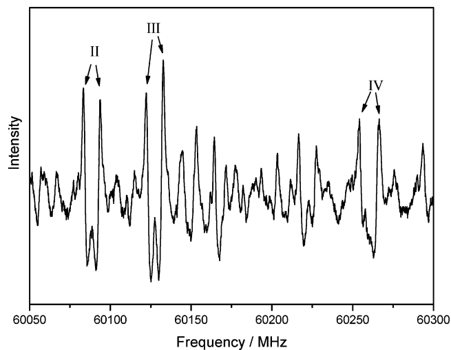
Figure 4. A portion of the RFWDR spectrum of J = 15 \leftarrow 14 transition of the ac conformer of H 2 C=CHSeCN obtained employing a radio frequency of 5.05 MHz. The spectrum shows the J = 15_6 \leftarrow 14_6 pair of lines associated with three of the five vibrational states that were assigned for this conformer. A Roman numeral indicates each state. Note the small intensity difference between states II and III.
