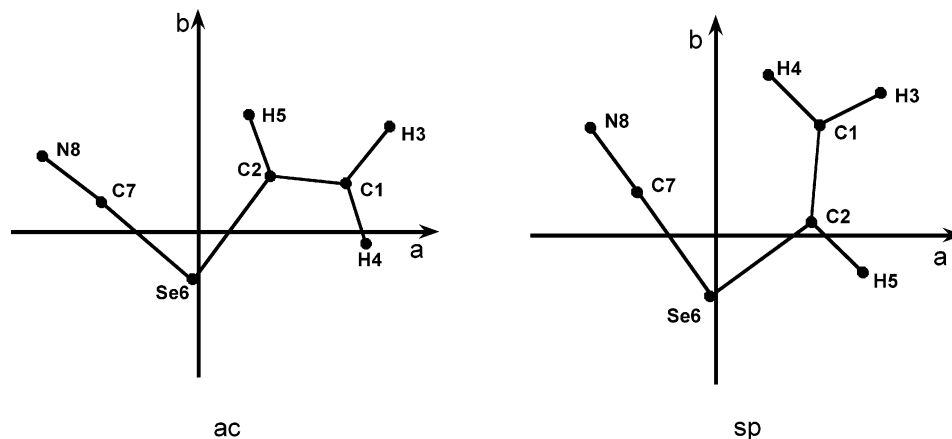
Figure 3. The ac and sp conformers of H 2 C=CHSeCN projected in the a – b principal inertial axis plane.
